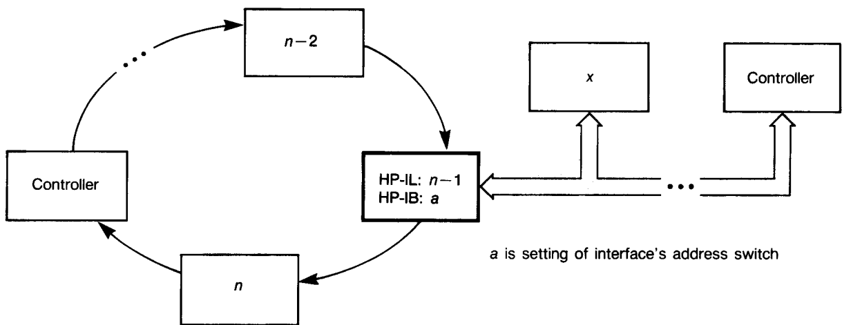
Addressing in Mailbox Mode
